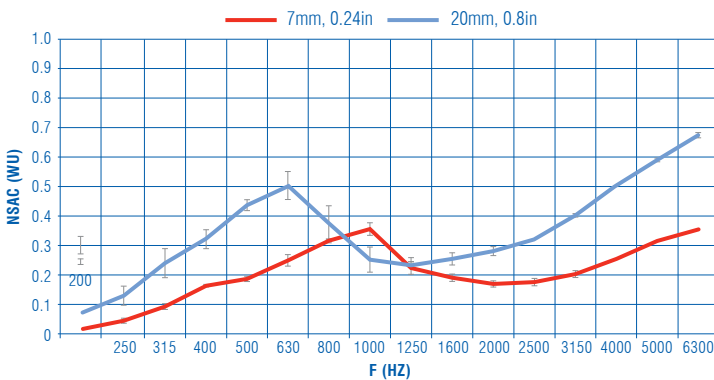
Felt*/0.2psf Film/Felt* Configuration Normal Incidence Sound Absorption Coefficient ASTM E1050-12 - ISO 10534-2
